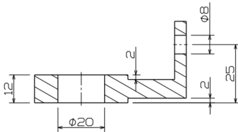
Section view A-A (1:1)
